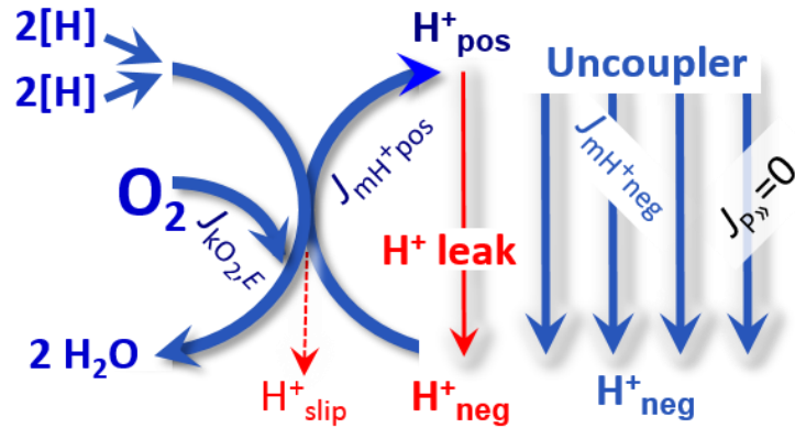
Fig. 6. ET-state: Noncoupled respiration, J_{kO_2,E} , is maximum at optimum exogenous uncoupler concentration and phosphorylation is zero, J_P = 0 . See also Fig. 2.
